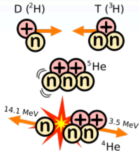
Deuterium-tritium (D-T) fusion reaction
